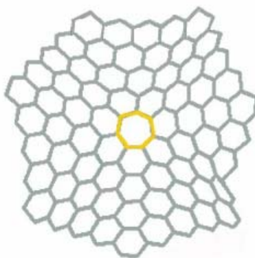
Figure 1. The One-Heptagonal Carbon Nanocone CNC_7[4] .
